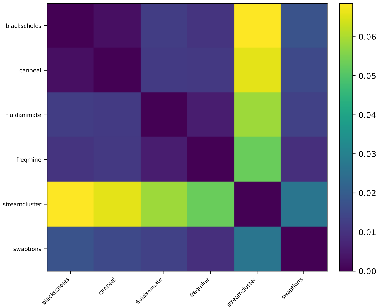
Cross-program phase-signature distance
