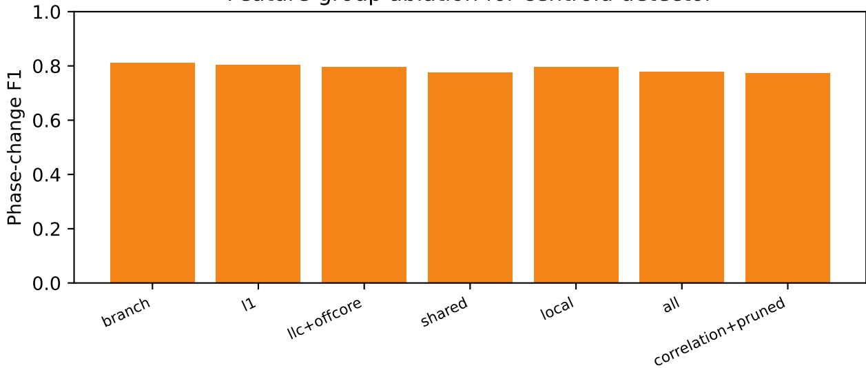
Feature-group ablation for centroid detector
