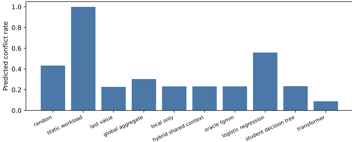
Trace-driven co-scheduling policy replay
