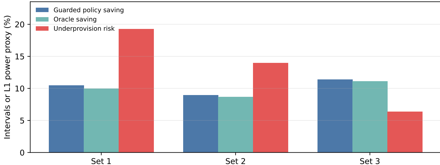
Small predicted-phase L1 control-policy simulation
