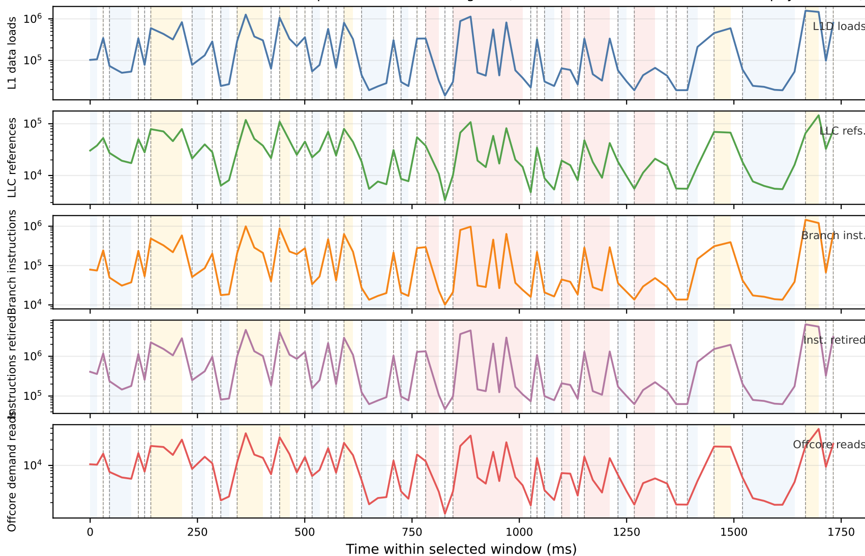
Raw selected-counter traces reveal repeated Phase 1/2/3 regions (Set 1, streamcluster, 16 threads, one physical core)
