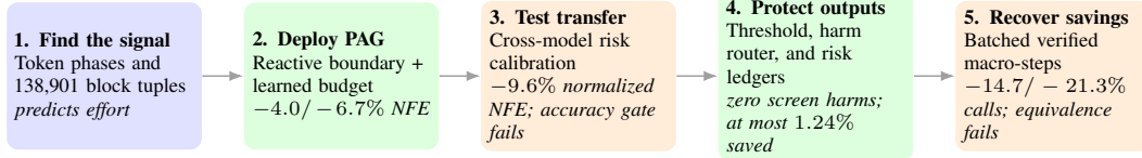
Figure 3: Approach progression. Each stage addresses the limitation exposed immediately before it; reported savings are relative to AdaBlock. The strongest corrected task result is PAG’s 6.7% NFE reduction on MATH-500 with a 1.33-point accuracy decrease. Larger apparent reductions fail either task-quality or exact-equivalence gates; output-preserving screens save at most 1.24%.
