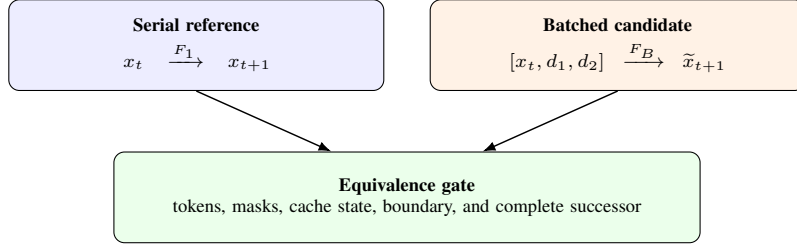
Figure 4: Exactness audit for verified macro-steps. A batched row is eligible only when it induces the same complete successor as the serial reference transition. The v8 pilot disagrees on 22 of 64 prompts, and v9 rejects the depth-dependent batch shape before rollout.
