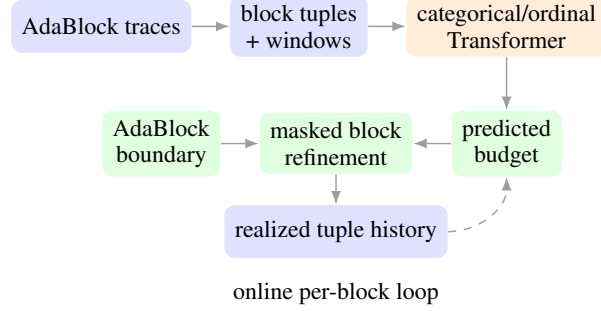
Figure 1: PAG separates two control signals. Current logits determine the next semantic boundary; history predicts a refinement budget. The realized tuple closes the loop only after the block is decoded.
