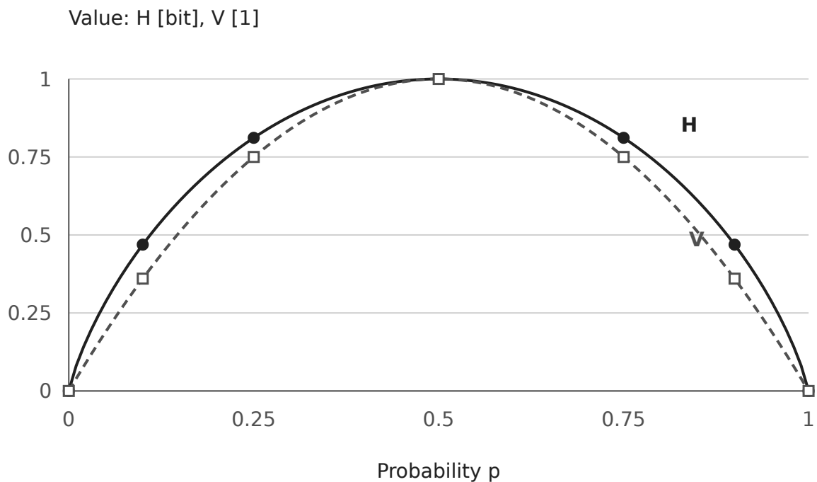
Figure 2. Entropy H in bits and normalized variance V without units. Both reach one at p = 1/2 . Lines are evaluated at increments of 0.01; the symbols identify the tabulated probabilities.
