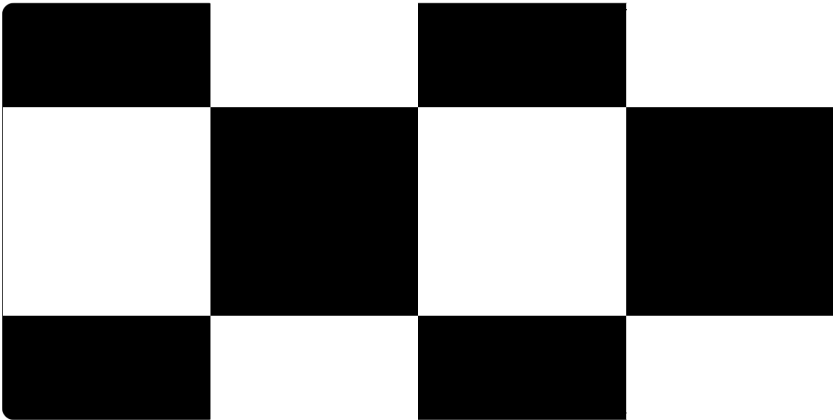
Figure 4. Thresholded probability field. Black means p \geq 1/2 ; white means p < 1/2 . This local PNG contains only black and white source pixels.
