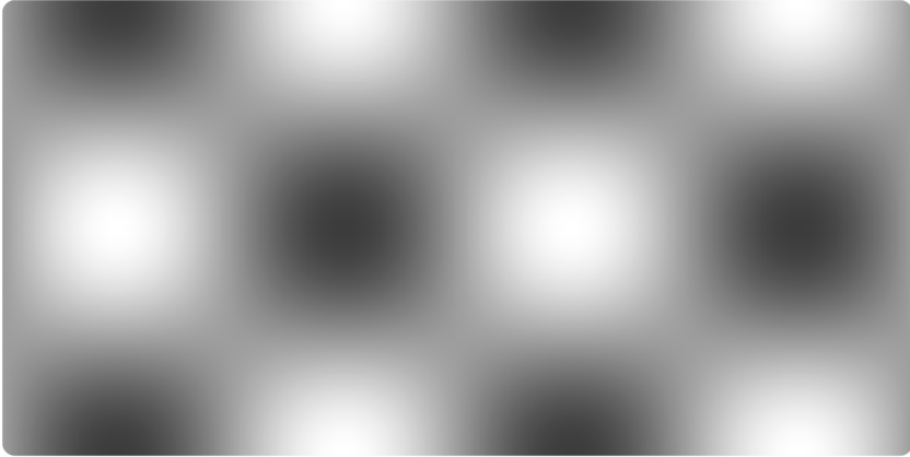
Figure 3. The same raster as Figure 1, rendered in grayscale. The spatial pattern remains, while the blue hue is removed.
