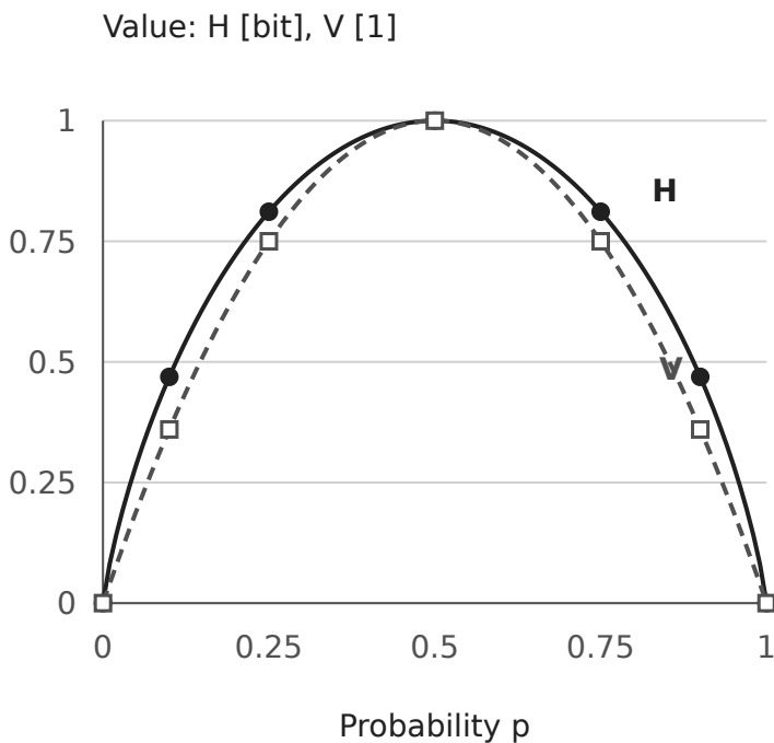
Figure 2. Entropy H in bits and normalized variance V without units. Both reach one at p = 1/2 . Lines are evaluated at increments of 0.01; the symbols identify the tabulated probabilities.
