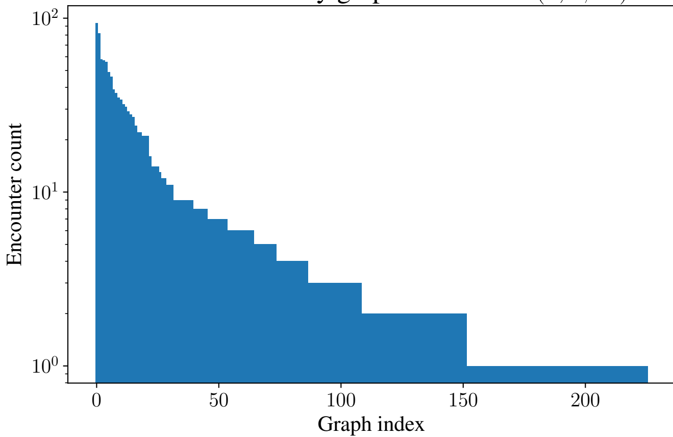
Encounter count by graph index for R(4, 4; 15)
