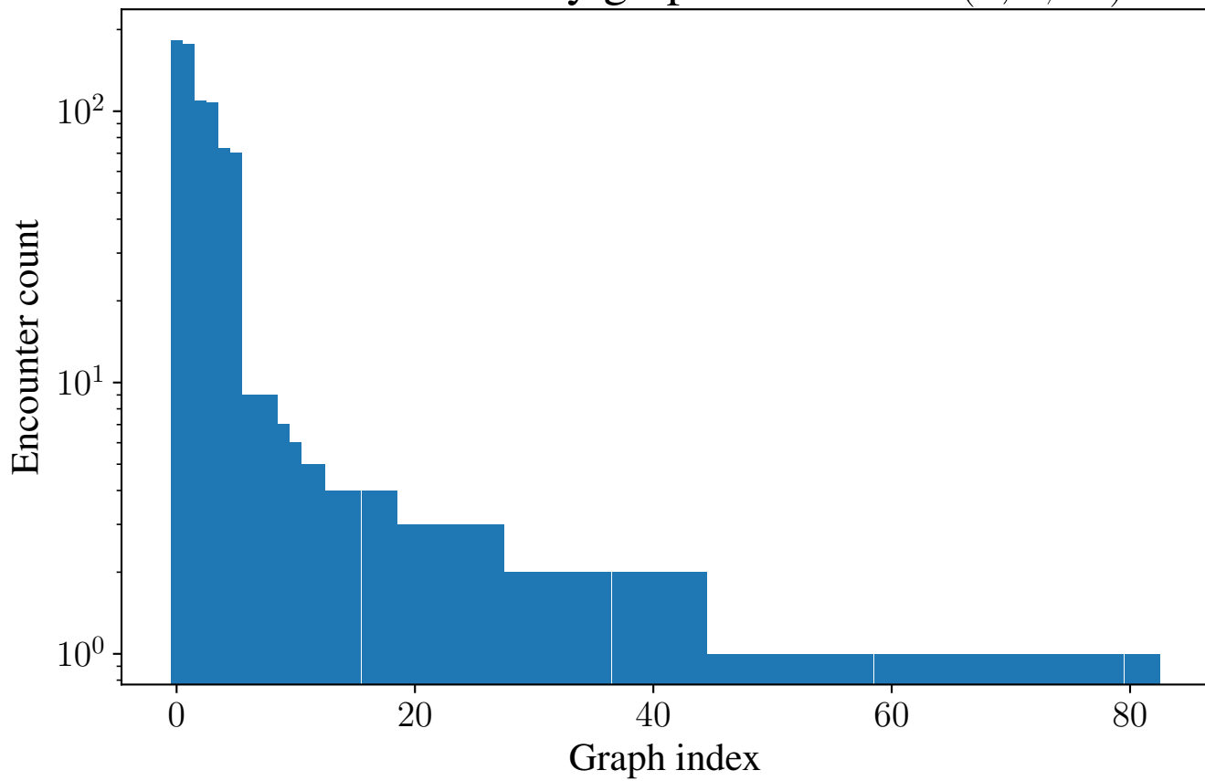
Encounter count by graph index for R(5, 5; 42)
