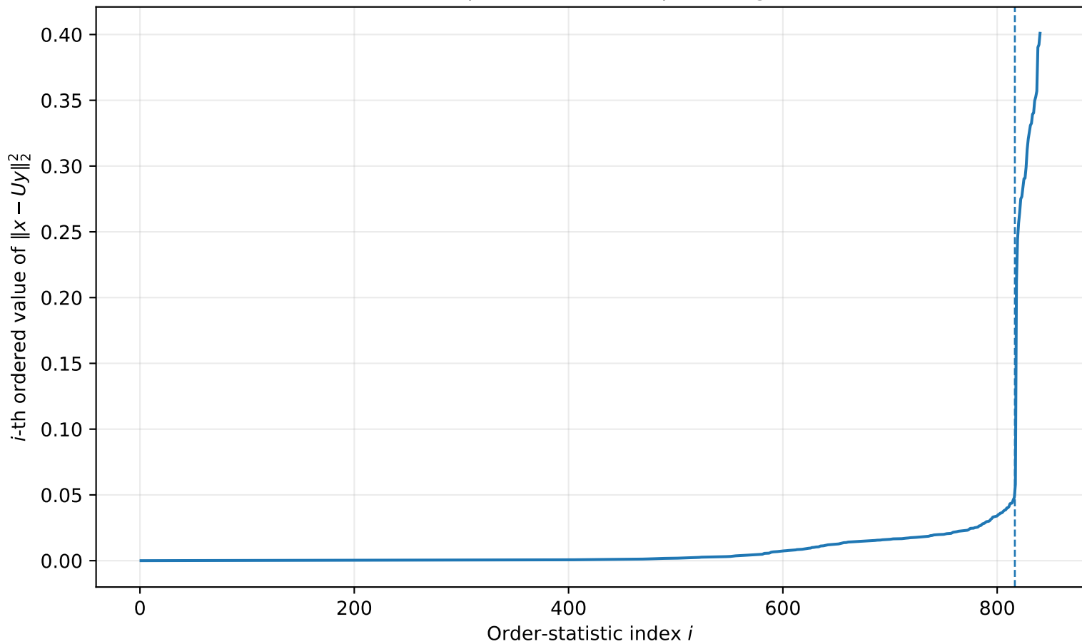
Canonical quaternionic 840-point alignment
