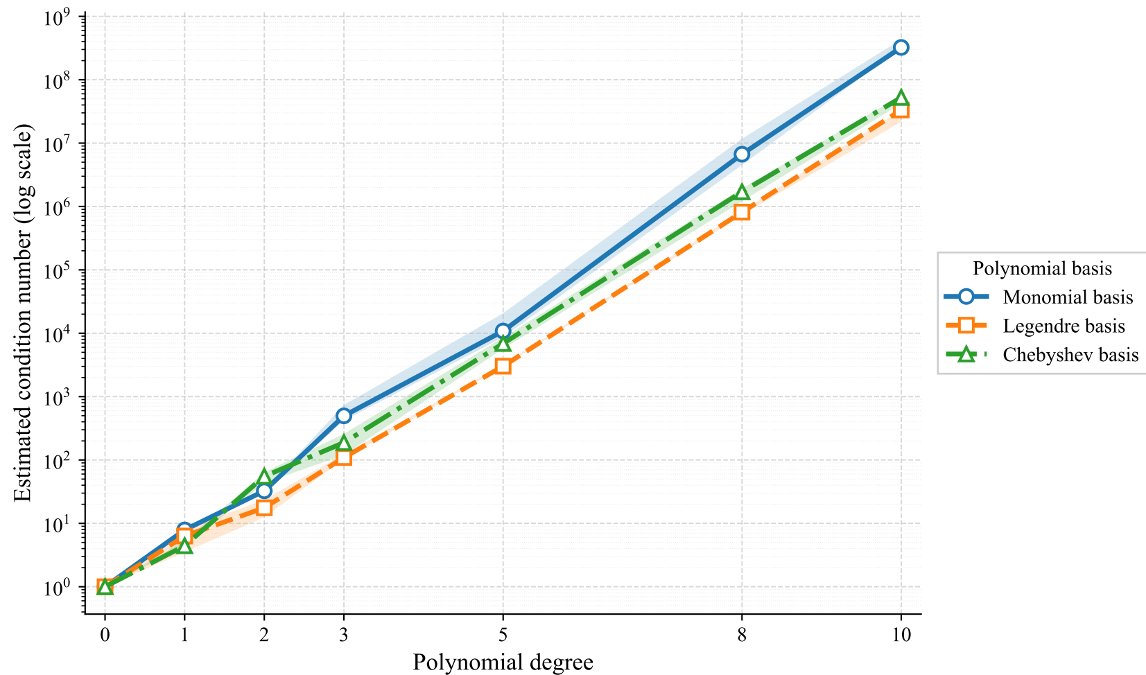
Estimated Condition Number versus Polynomial Degree
