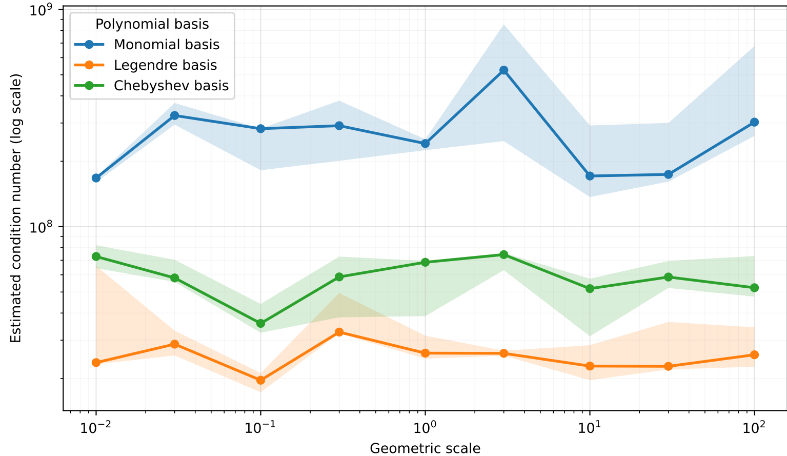
Estimated Condition Number versus Geometric Scale
