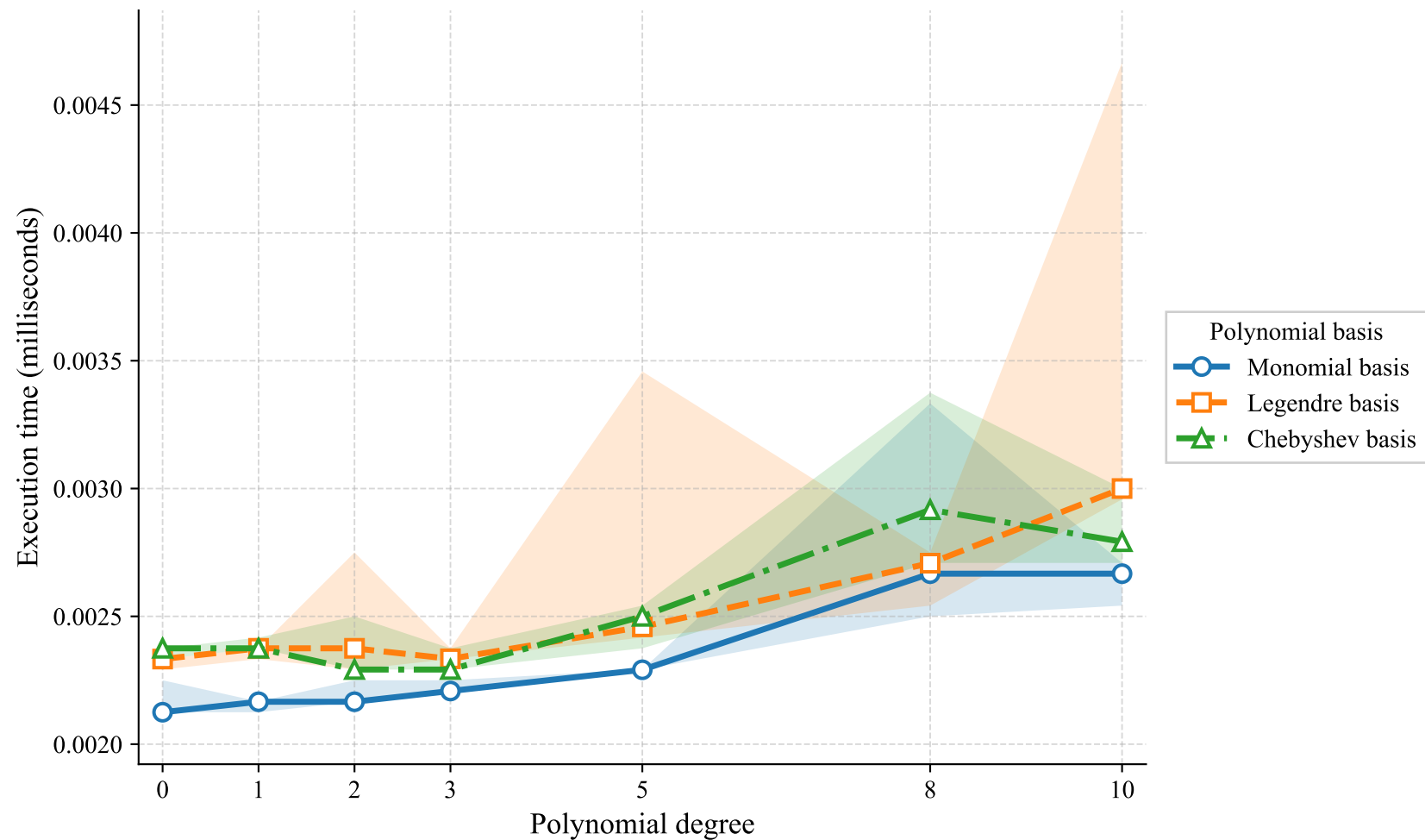
Execution Time versus Polynomial Degree
