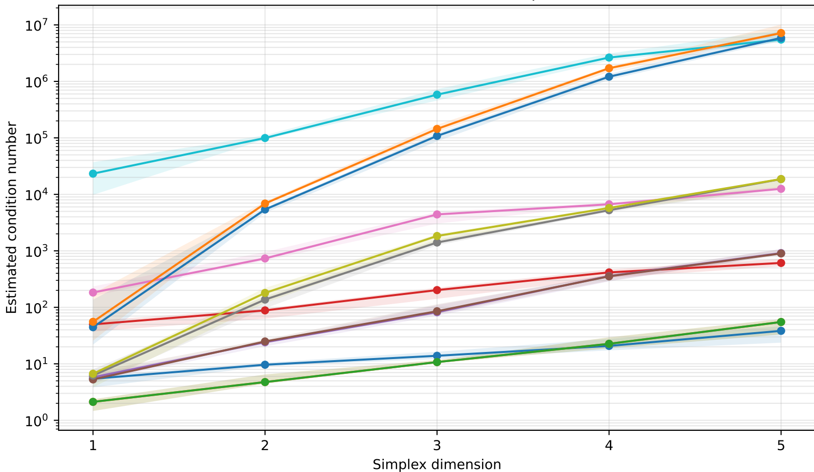
Condition number as a function of simplex dimension
