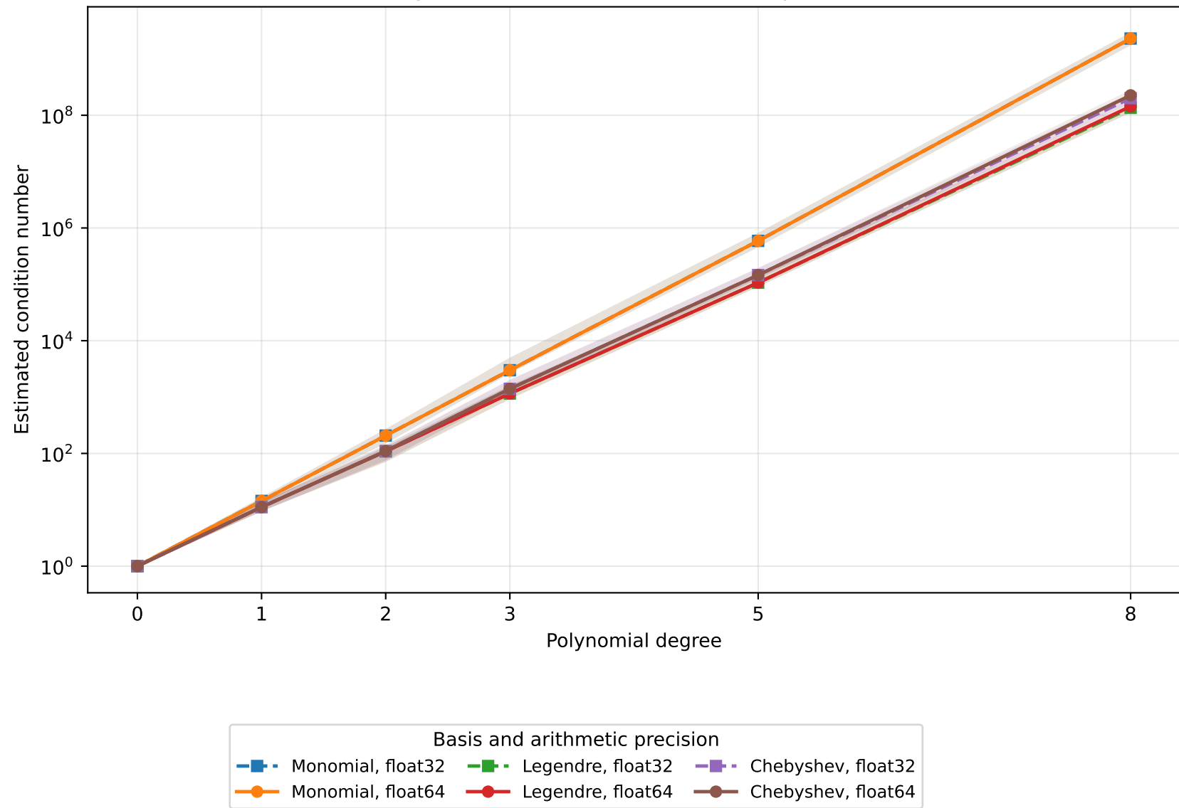
Conditioning under float32 and float64 (simplex dimension 3)
