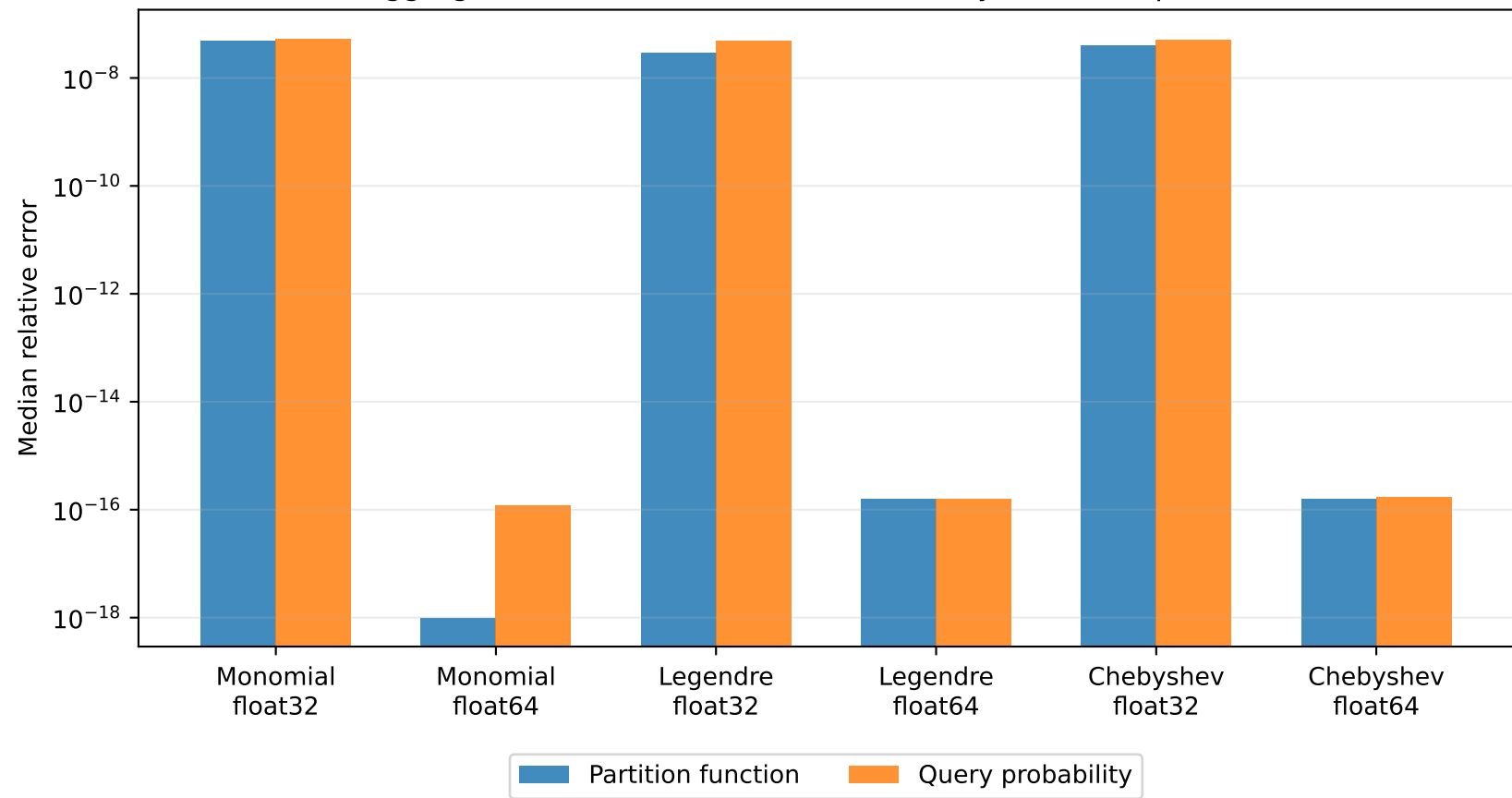
Aggregate downstream numerical error by basis and precision
