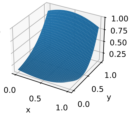
source degree 3, trial 1
