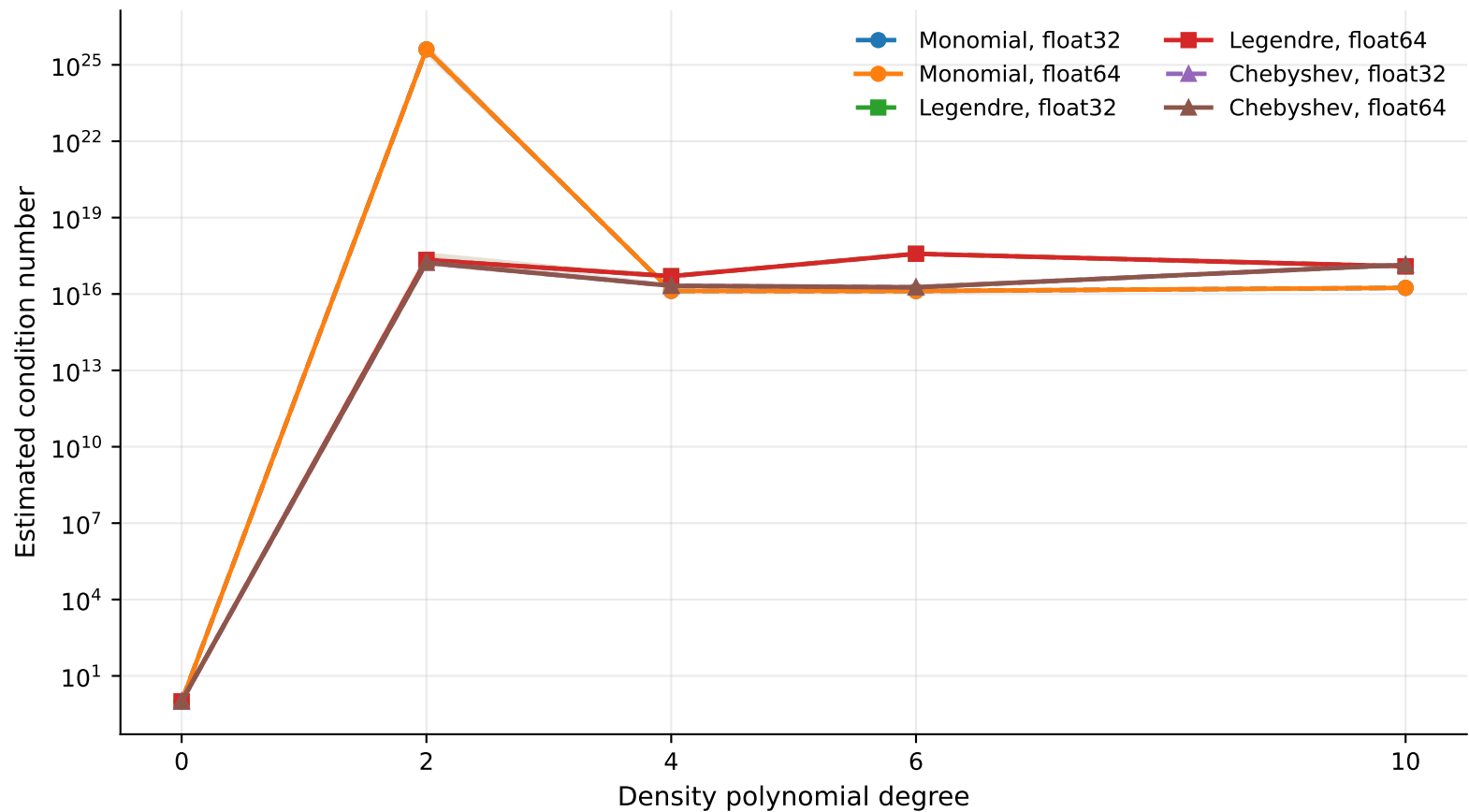
Basis condition number versus polynomial degree dimension 3
