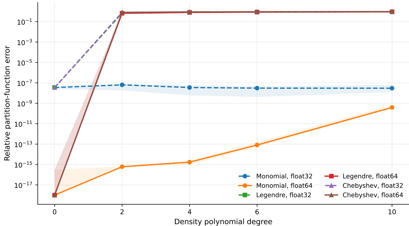
Partition-function relative error versus polynomial degree dimension 3
