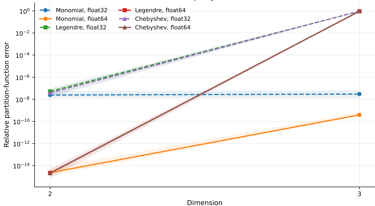
Partition-function relative error versus dimension density degree 10
