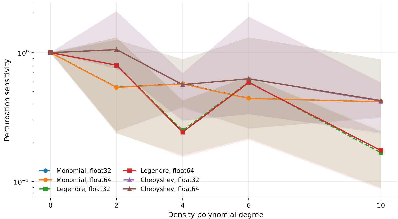
Perturbation sensitivity versus polynomial degree dimension 3
