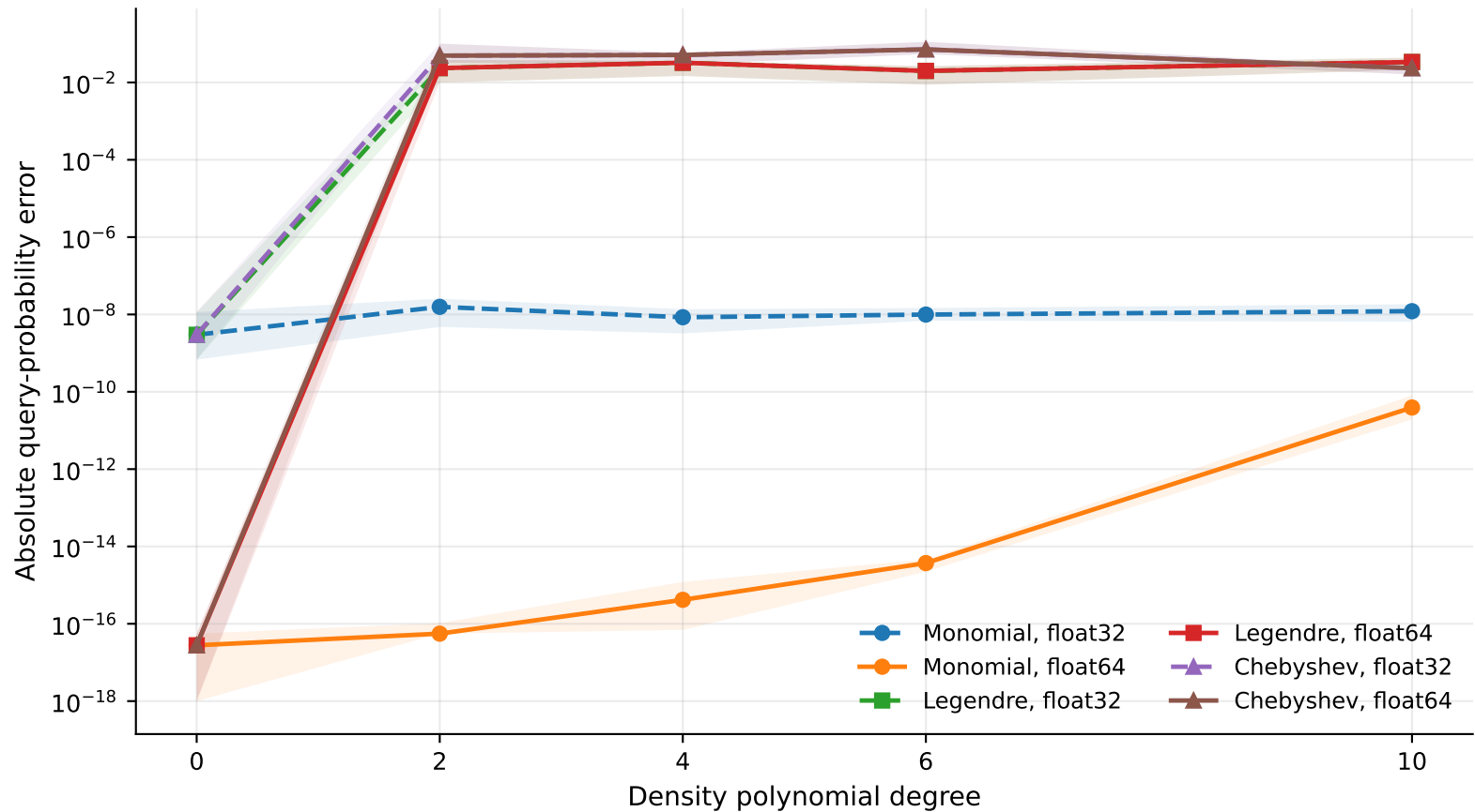
Query-probability absolute error versus polynomial degree dimension 3
