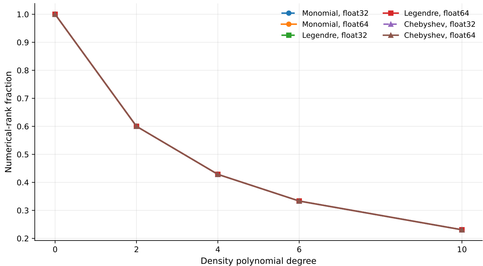
Retained numerical-rank fraction versus polynomial degree dimension 3
