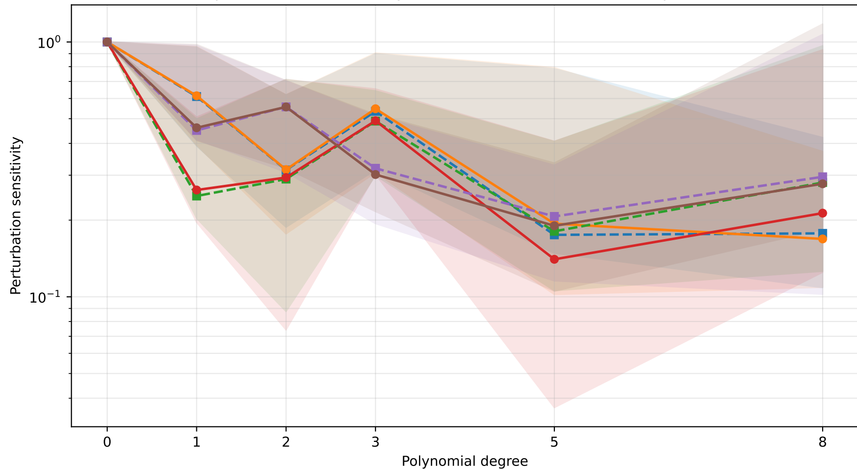
Coefficient-perturbation sensitivity under float32 and float64 (simplex dimension 3)
