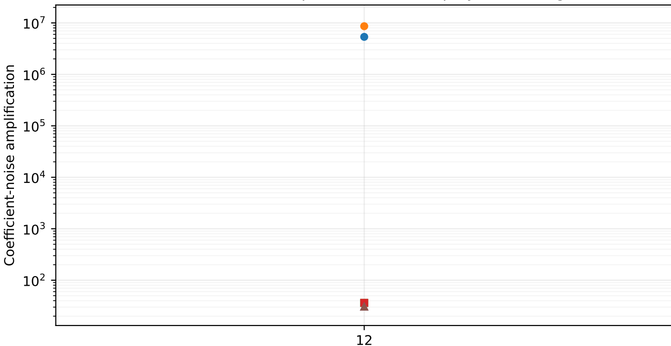
Coefficient-noise amplification versus polynomial degree
