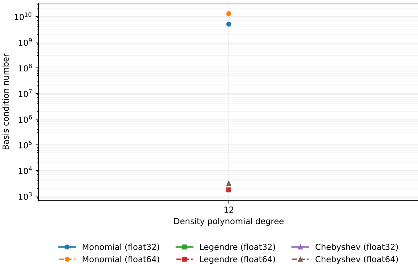
Basis condition number versus polynomial degree
