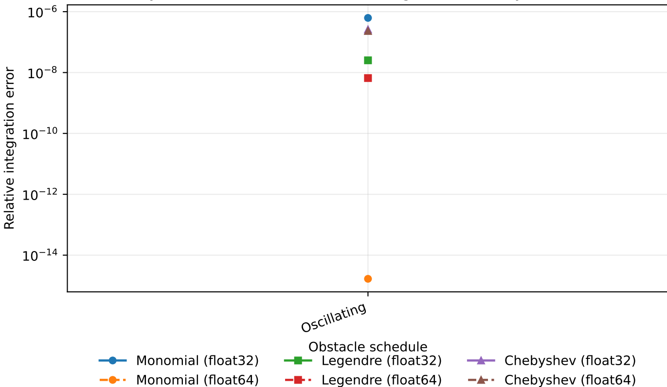
Dynamic constrained-domain integration error by schedule
