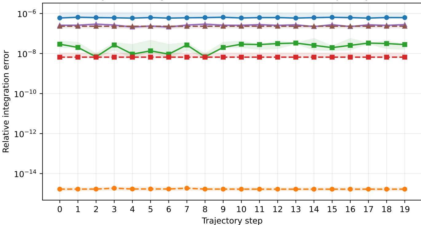
Dynamic integration error across the obstacle trajectory
