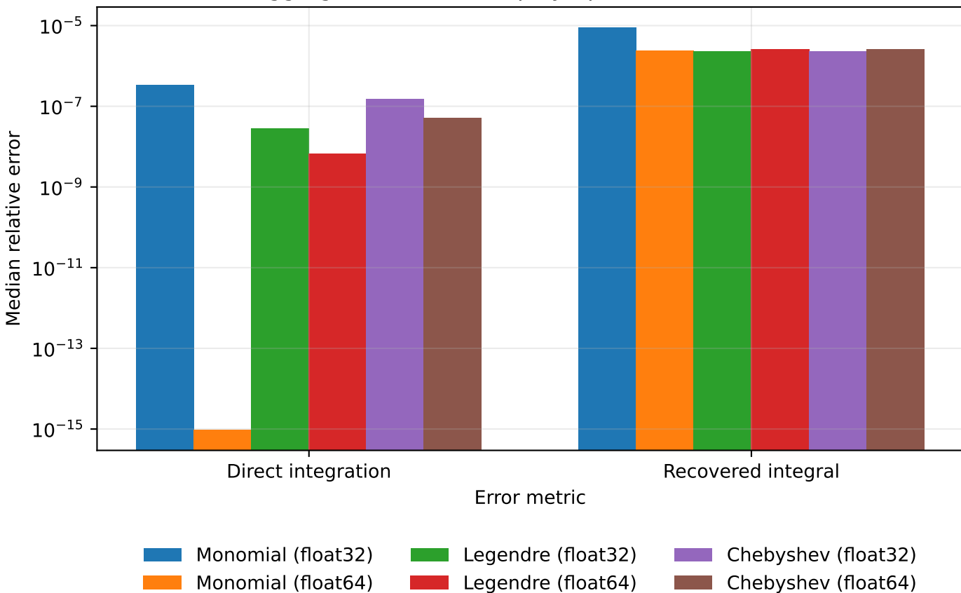
Aggregate constrained-polytope numerical errors
