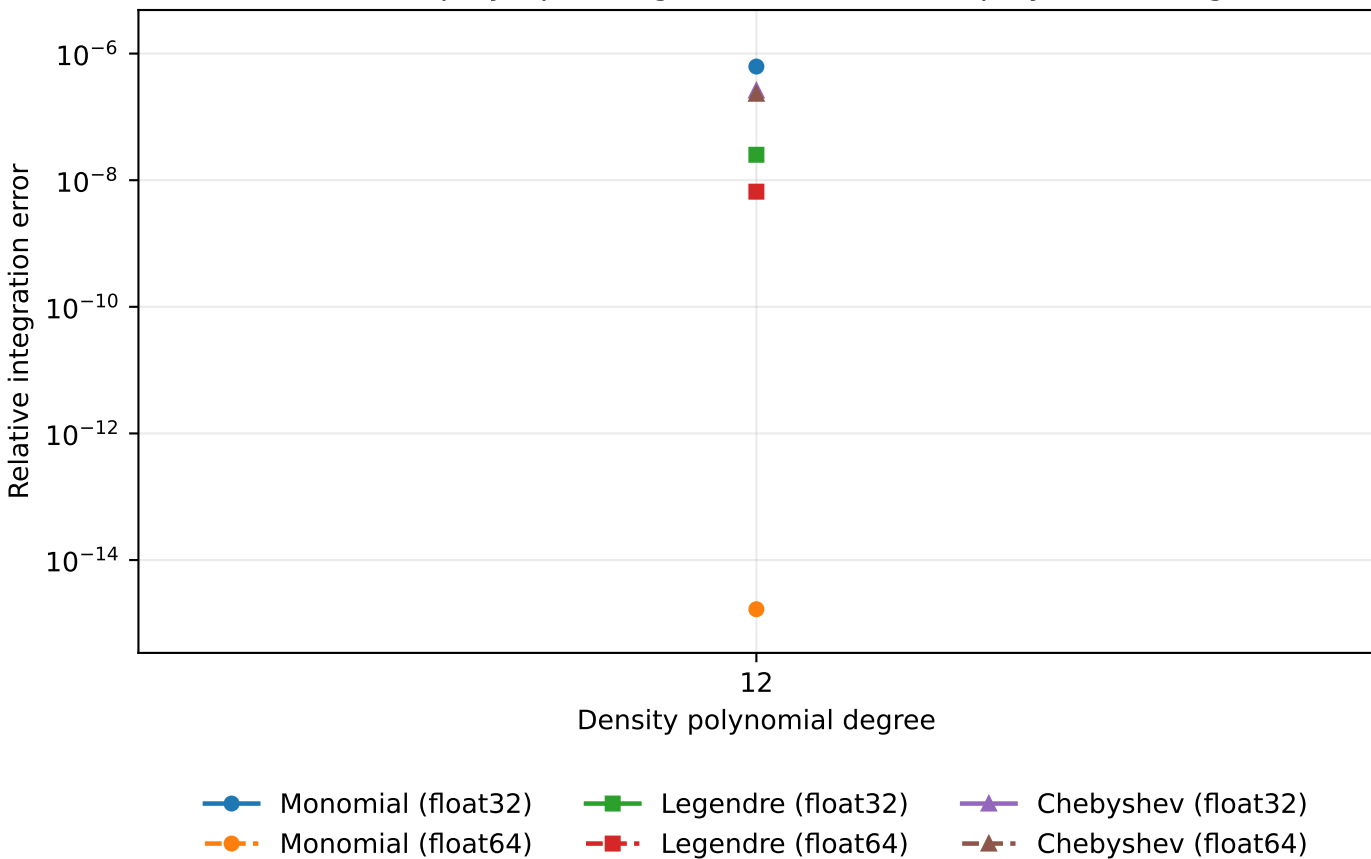
Constrained-polytope integration error versus polynomial degree
