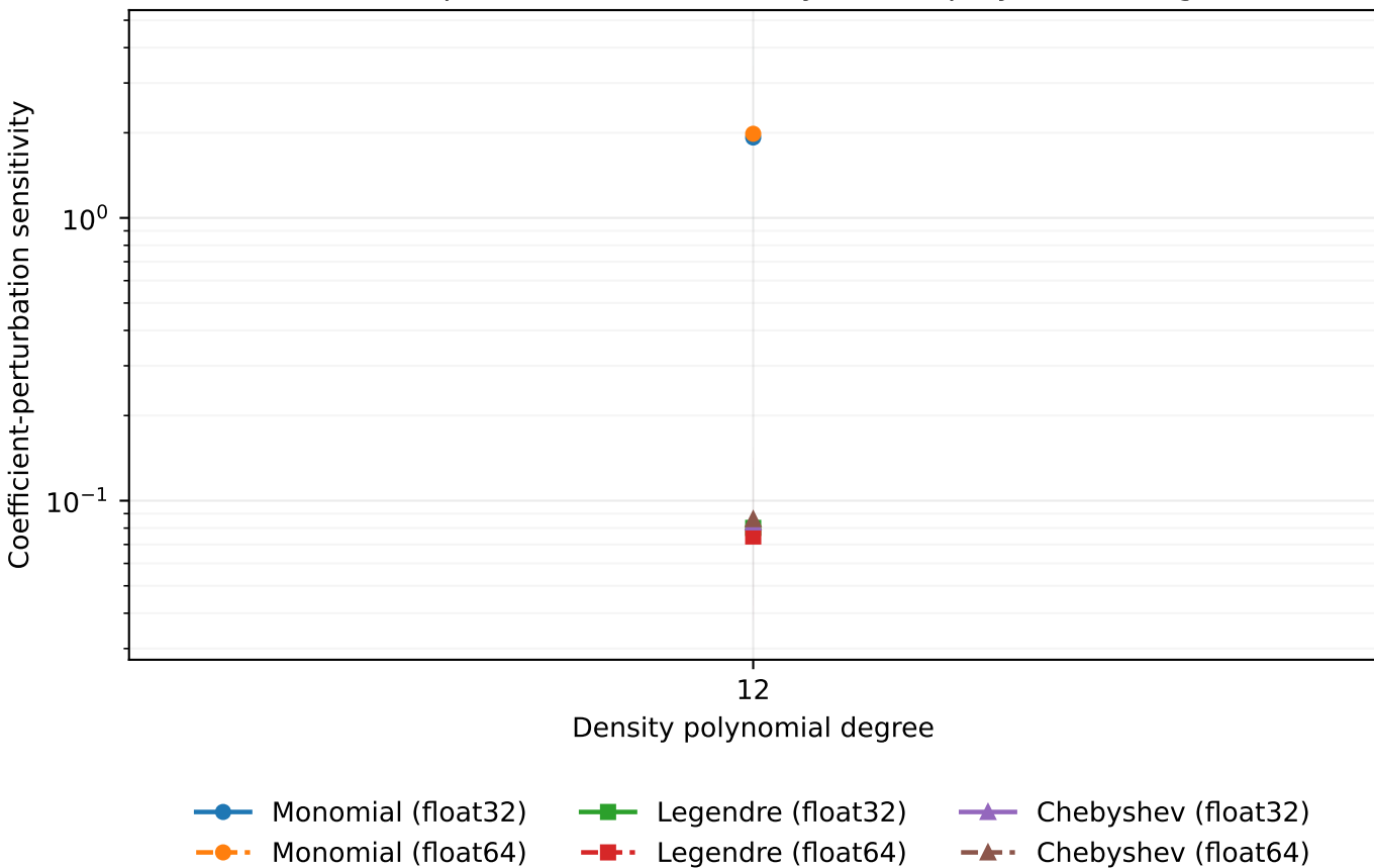
Coefficient-perturbation sensitivity versus polynomial degree
