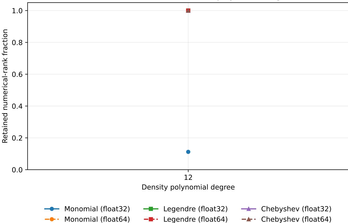
Retained numerical rank versus polynomial degree
