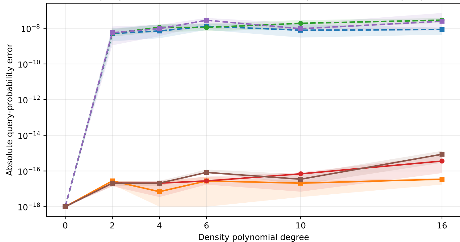
Downstream query error under float32 and float64 (simplex dimension 3, query scale 0.5)
