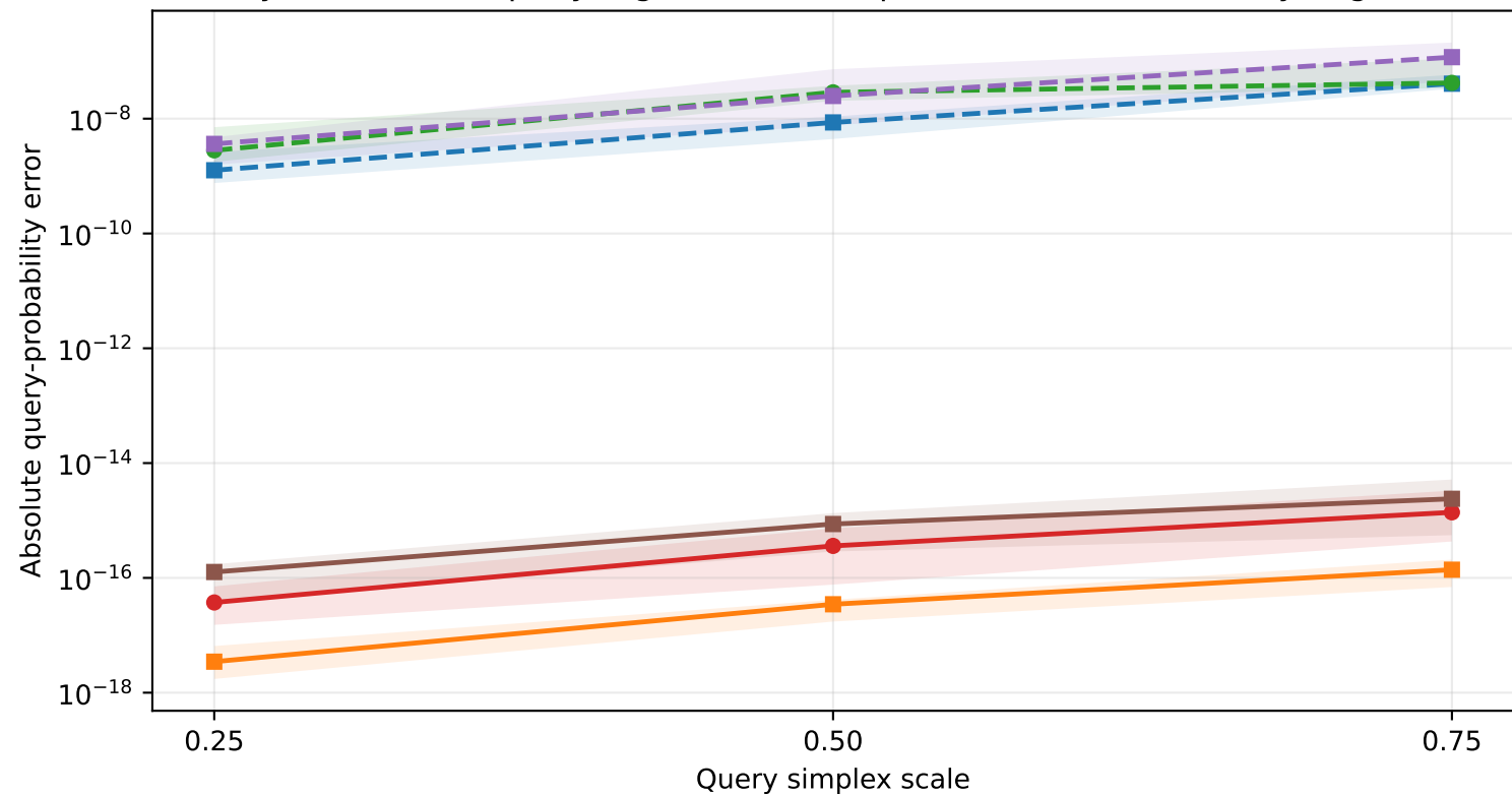
Query error versus query-region scale (simplex dimension 3, density degree 16)
