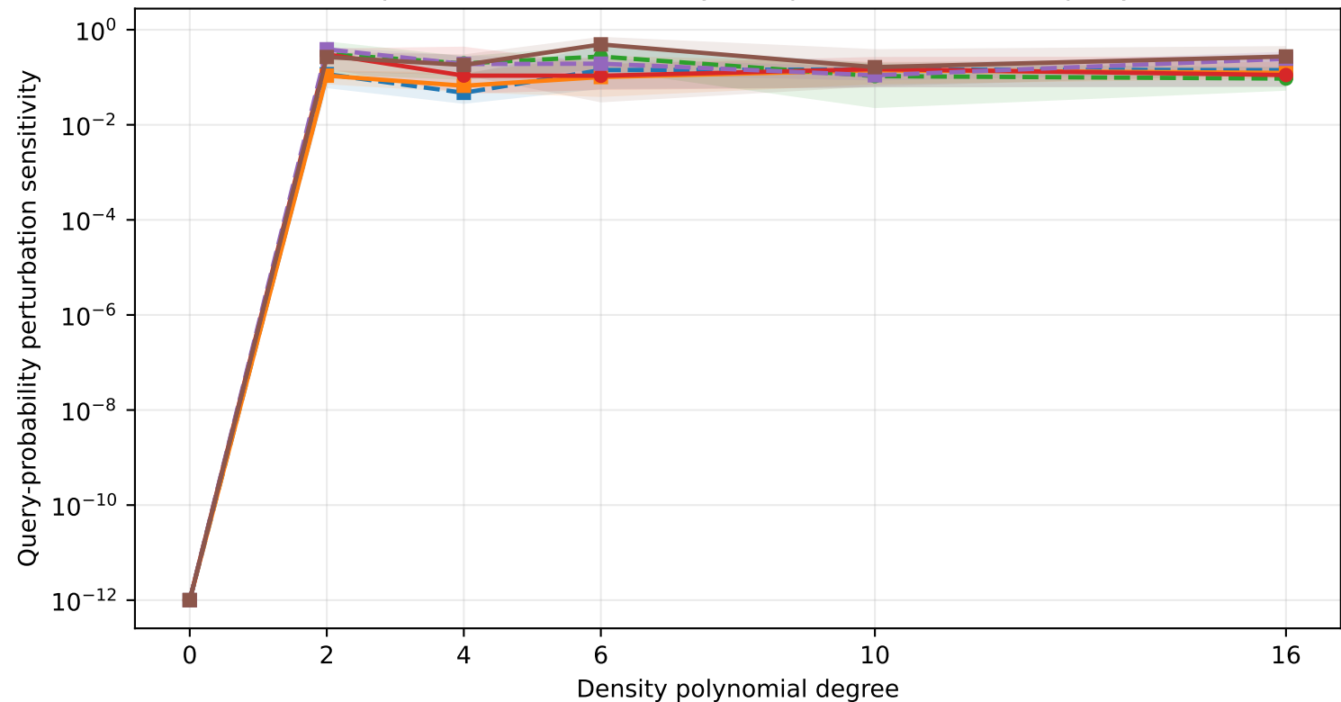
Downstream perturbation sensitivity (simplex dimension 3, query scale 0.5)
