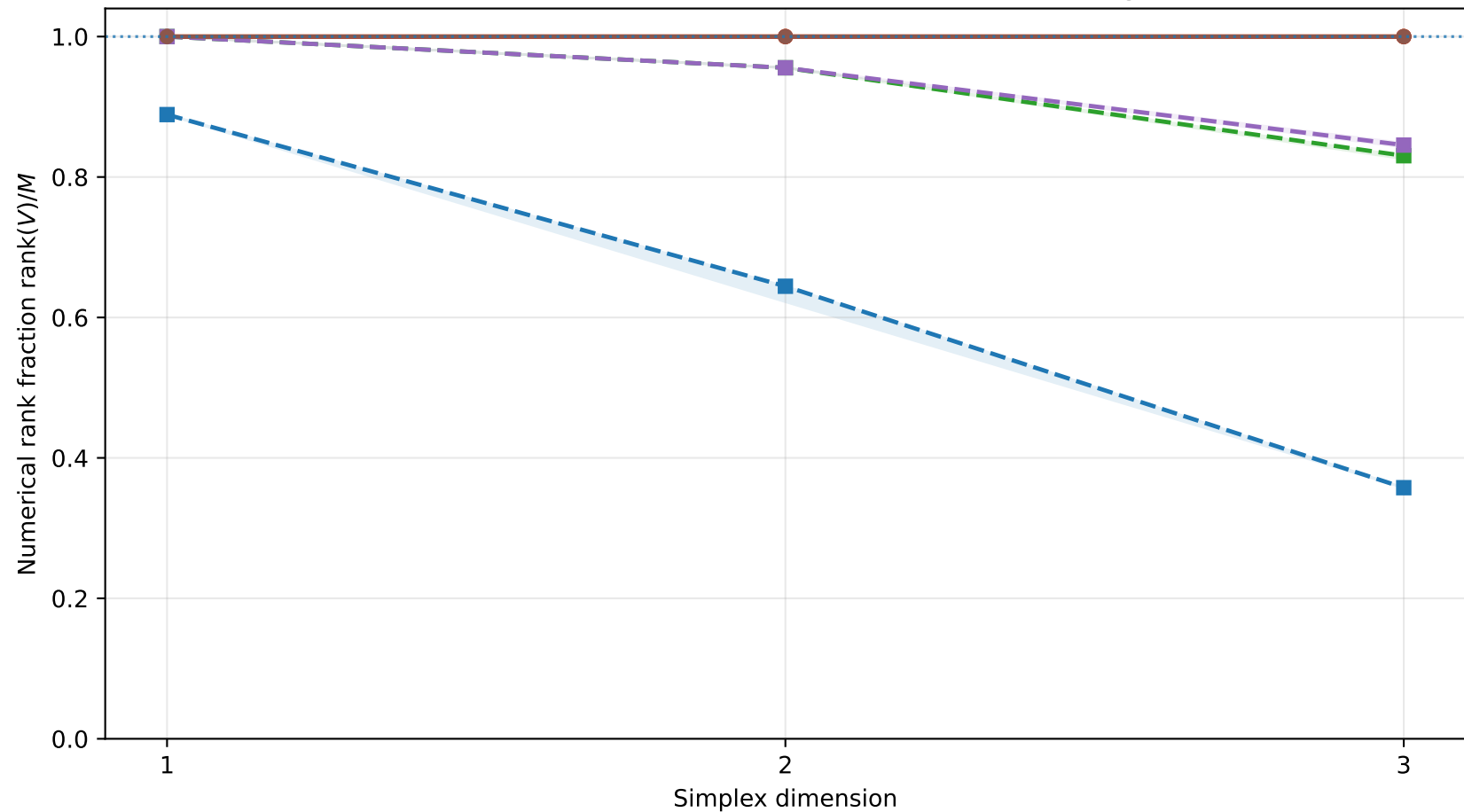
Numerical rank retained under float32 and float64 (degree 8)
