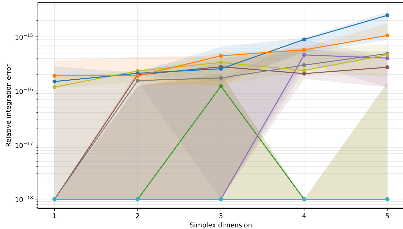
Relative integration error as a function of simplex dimension
