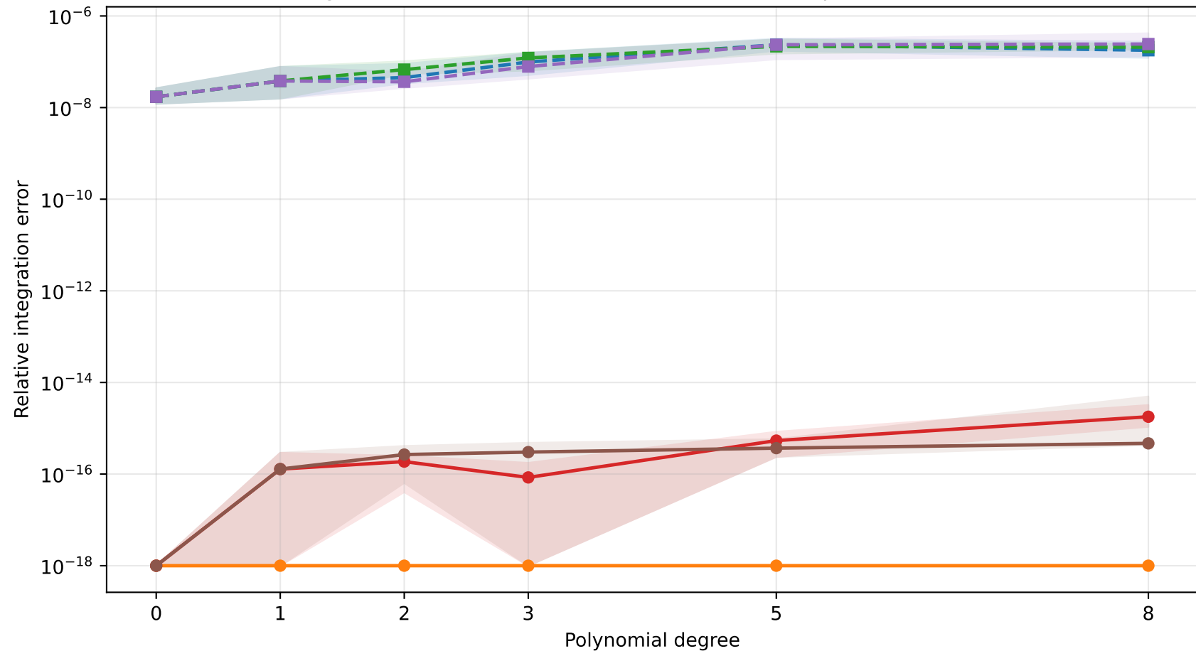
Integration error under float32 and float64 (simplex dimension 3)
