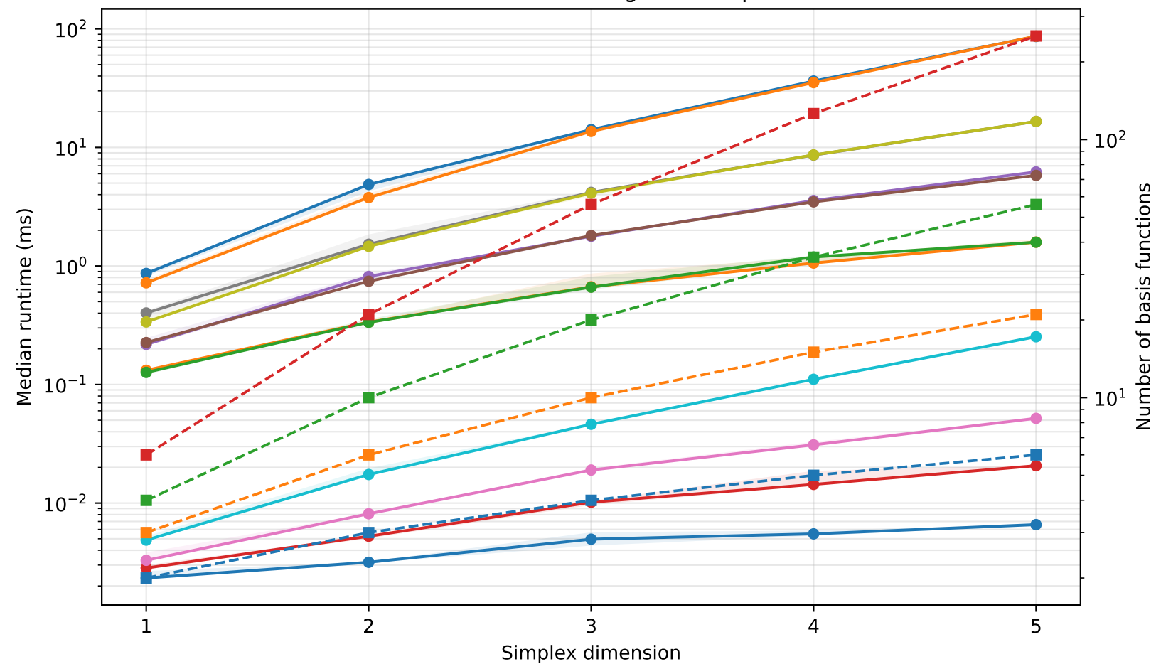
Runtime and basis-count scaling with simplex dimension
