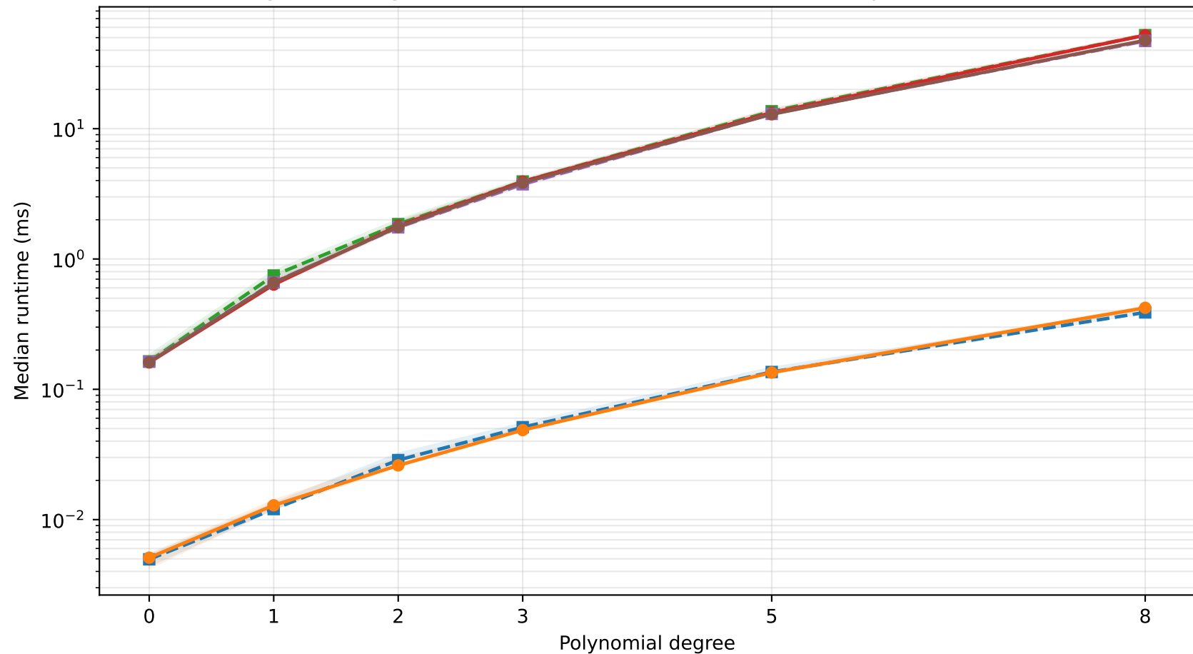
Integration-stage runtime under float32 and float64 (simplex dimension 3)
