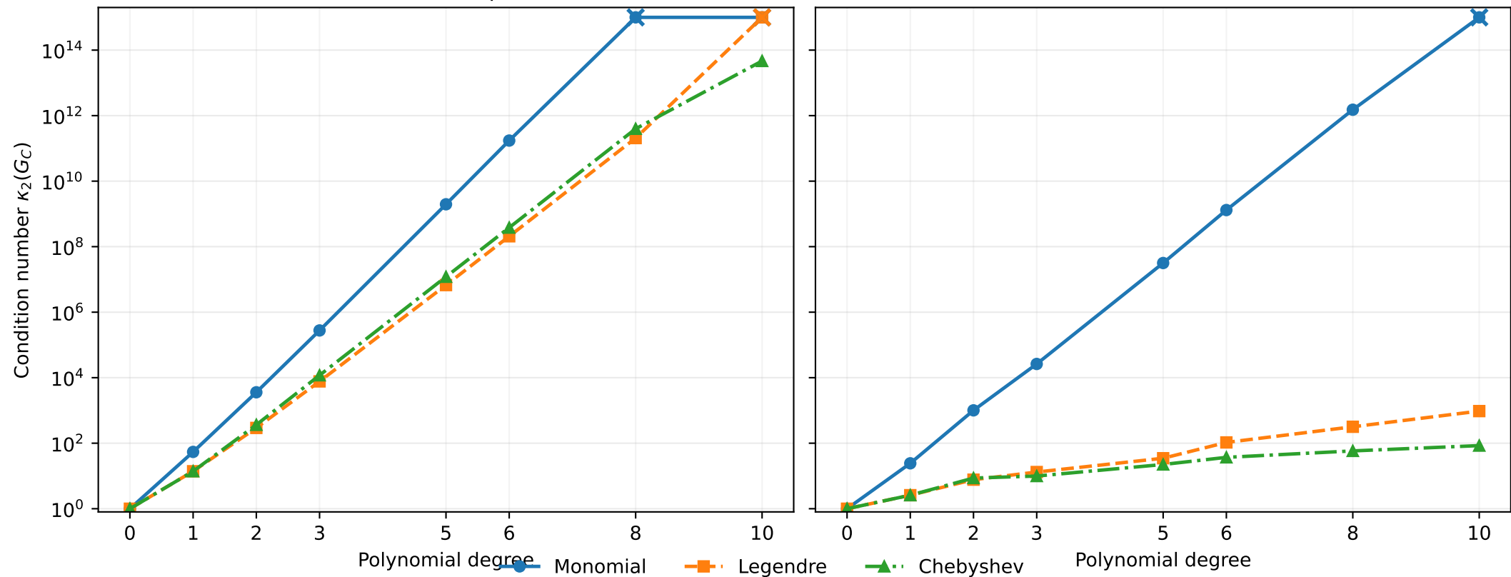
Conditioning of the constraint-induced integration matrix G_C in dimension 2 (a) Unit simplex (b) Box with obstacle
