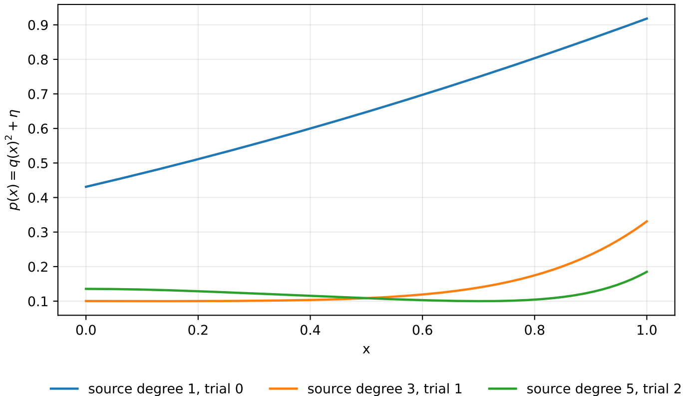
Representative generated one-dimensional densities
