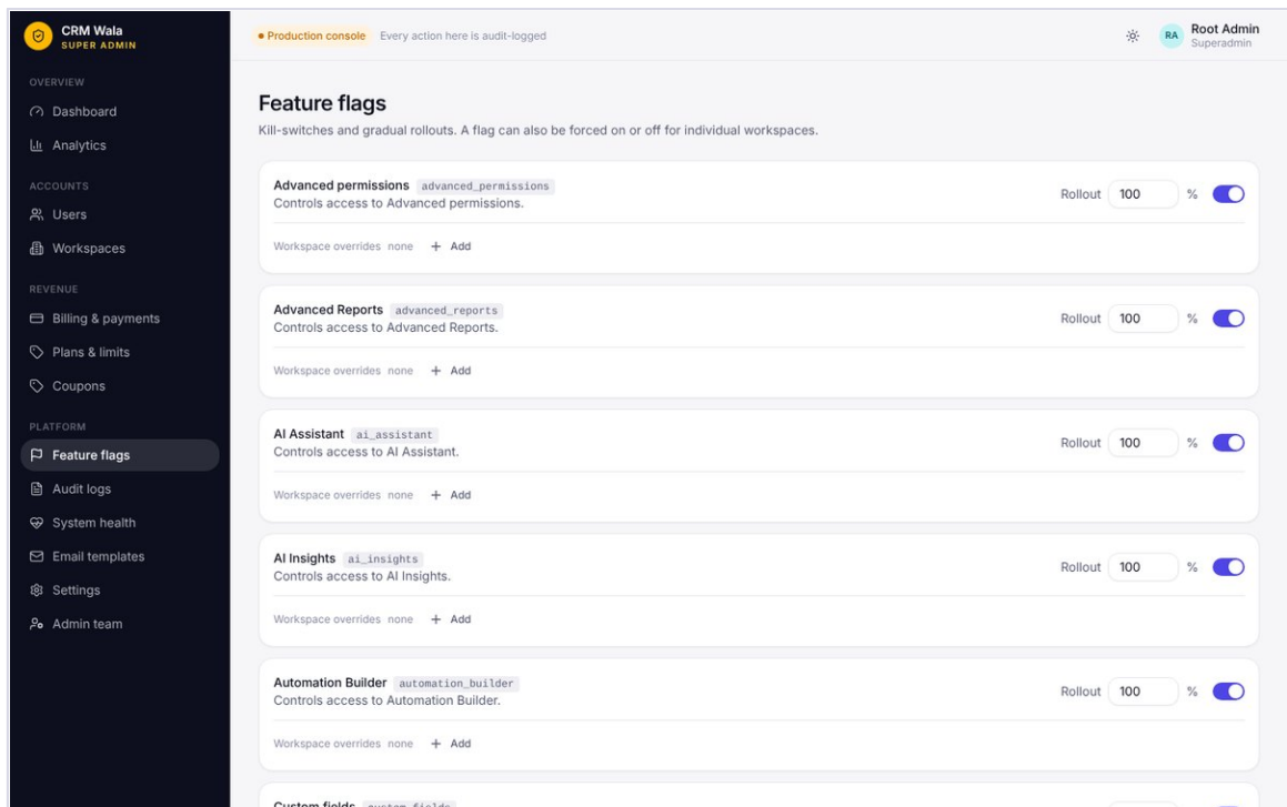
Figure 38. Feature flags.
