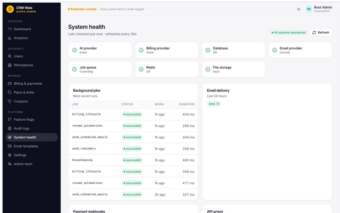
Figure 40. System health.
