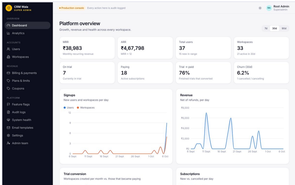
Figure 31. Platform overview.
