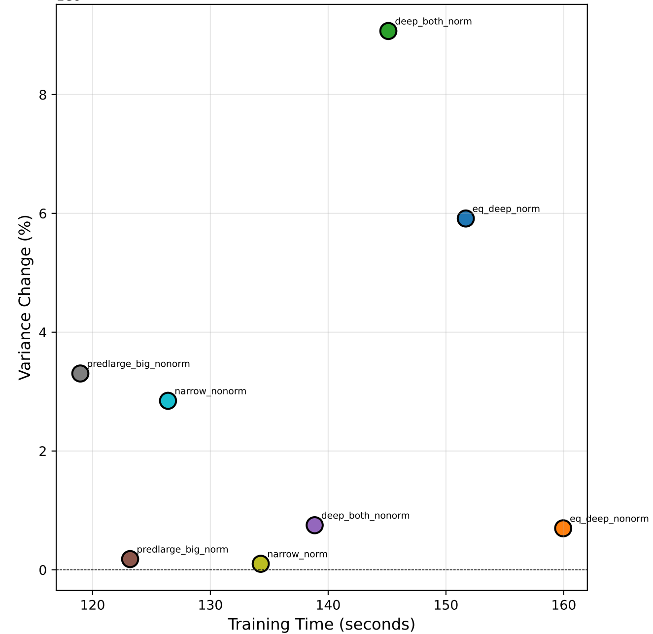
Time vs Performance Trade-off
