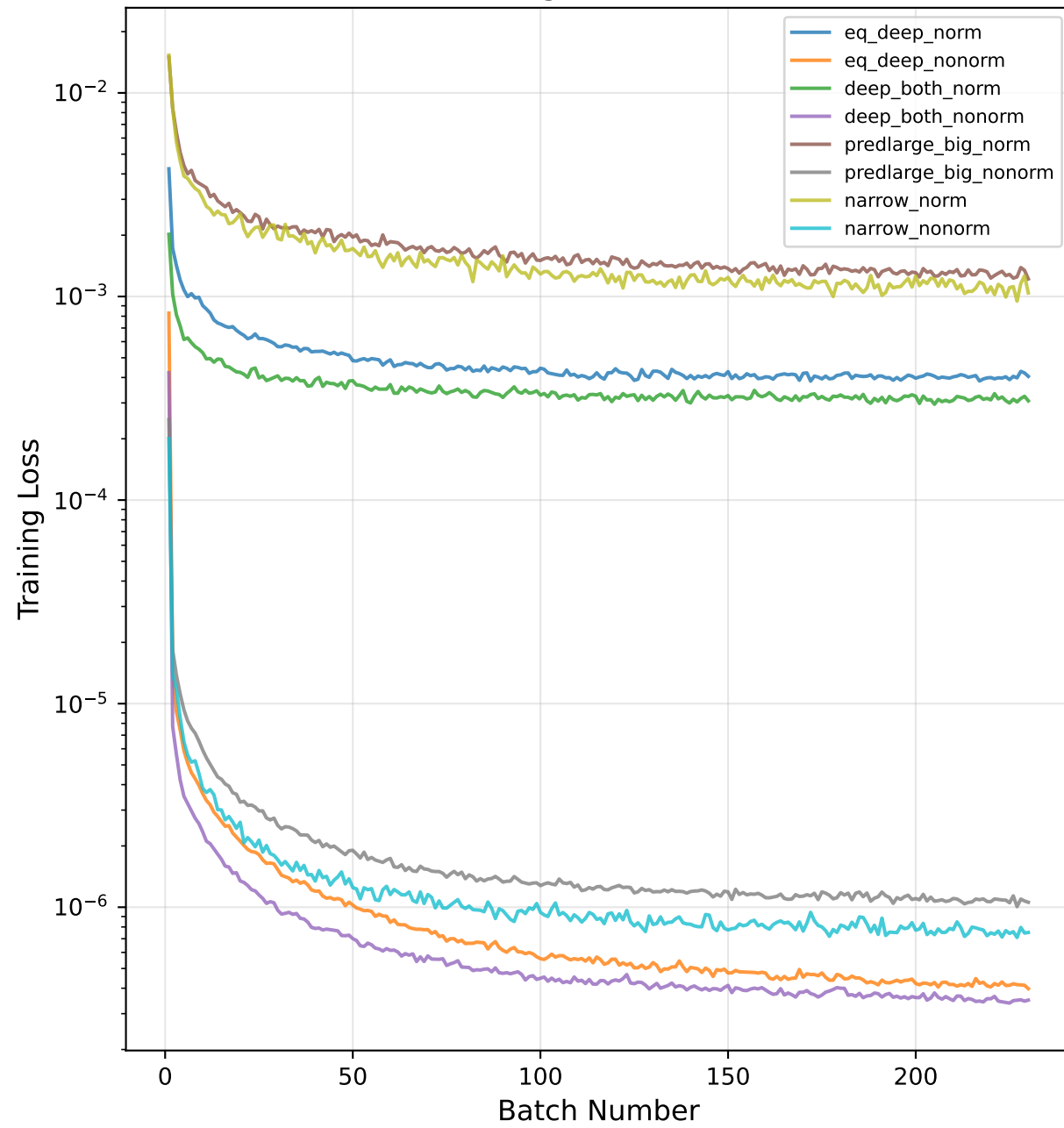
Training Loss Curves
