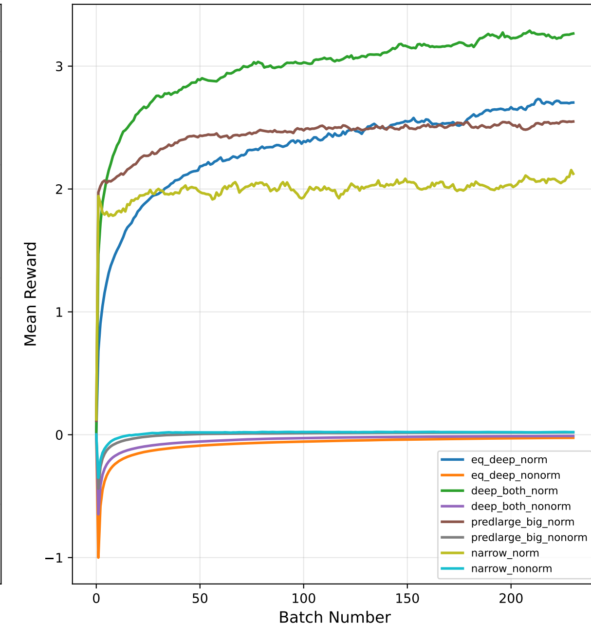
Mean Reward Evolution
