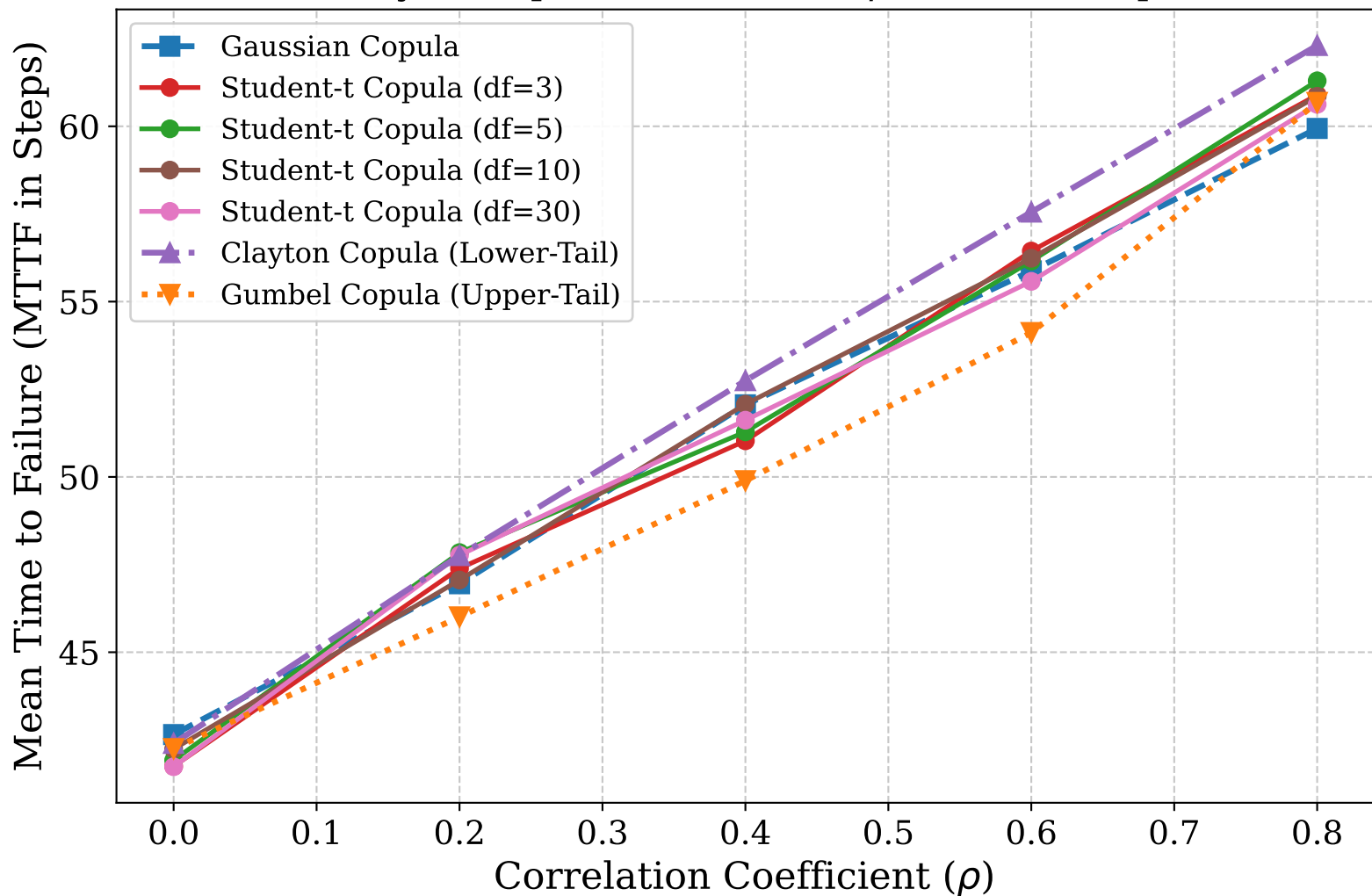
MTTF Sensitivity to Copula Correlation ( \rho ) and Tail Dependence ( df )
