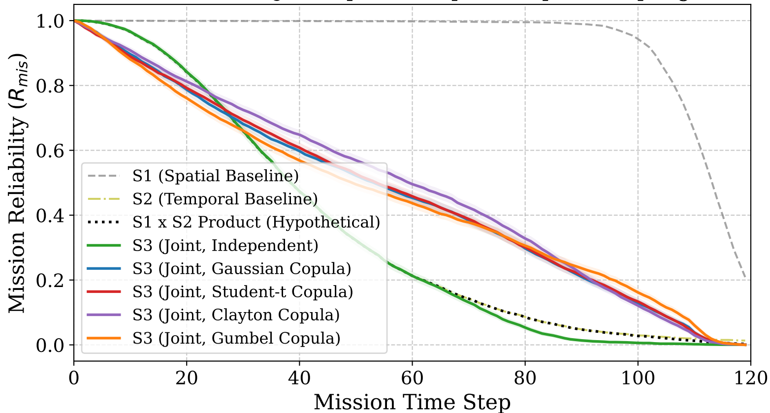
Scenario S3: Joint Spatio-Temporal Copula Coupling
