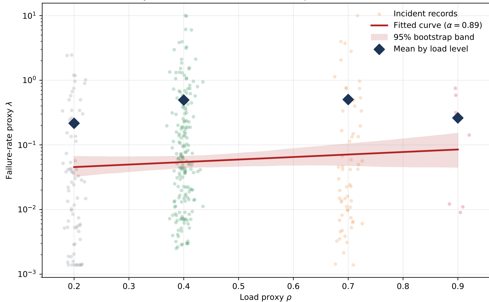
Proxy-based calibration of the load-dependent failure model
