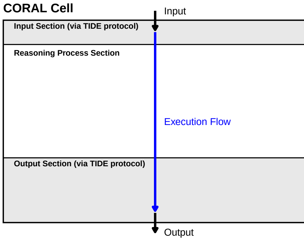
Figure 3: Conceptual structure of a CORAL Cell, illustrating its input-output oriented design, explicit reasoning process, and TIDE protocol integration.
